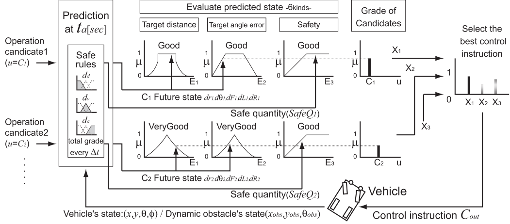
Figure 4: Predictive fuzzy controller
