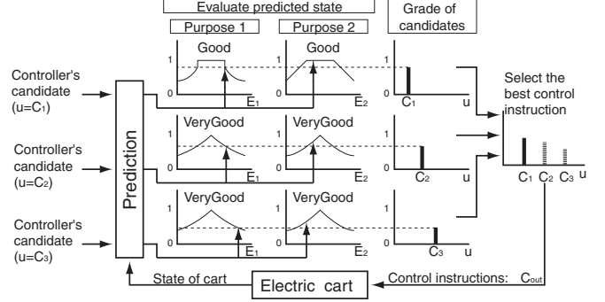
Fig. 6. Overview of predictive fuzzy control.
