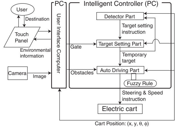
Fig. 1. System configuration.
