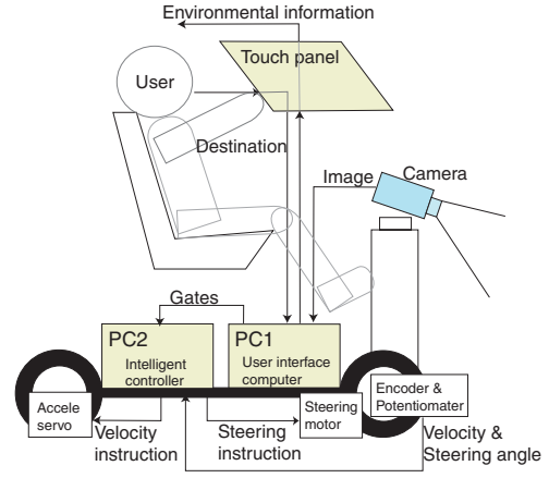
Fig. 7. Hardware construction of the system.
