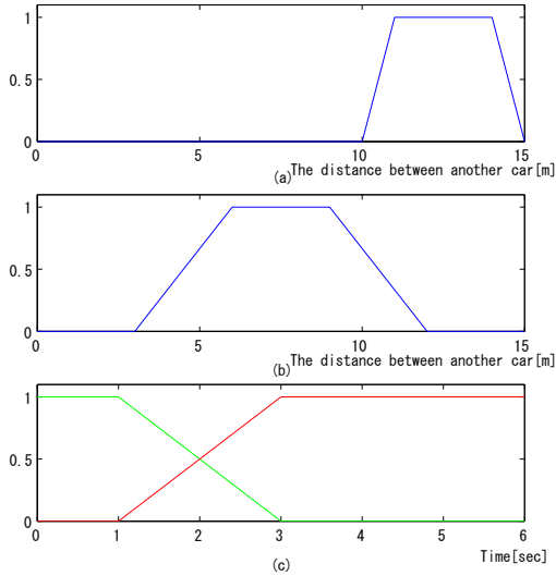
Fig. 4. The example of the auxiliary sets of the simple time-change fuzzy set
