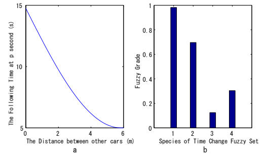
Fig. 6. The comparison of degrees
