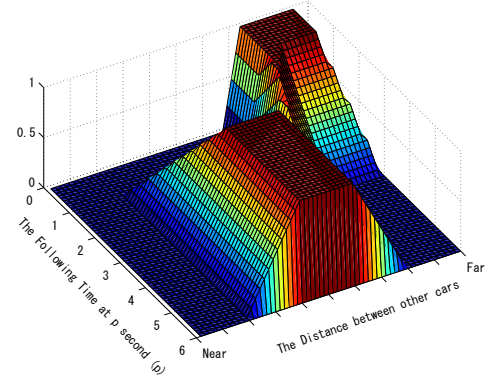
Fig. 5. The example of the membership function of the simple time-change fuzzy sets
