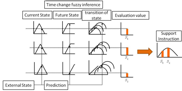
Fig. 2. An example of the time-change fuzzy set
